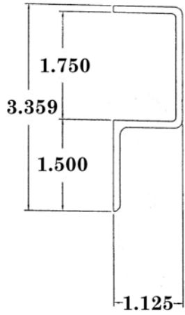
Part C-531 - Top Rail
