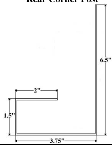
Part GR3-1 (108'')- Grumman Rear Corner Post
