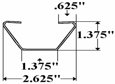
Part 419-1D (92.5) & 419-1E (98.5)- Roof Bow Grumman
