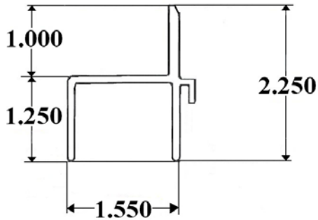
Part 02020- Supreme Front Vertical & Horizontal Connector VA & IA
