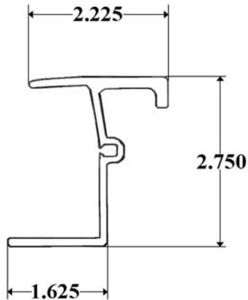
Part 3009- Utilimaster Rear Top Rail
