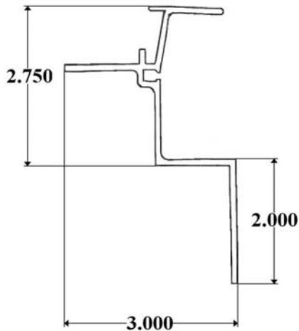
Part 3002- Utilimaster Top Rail
