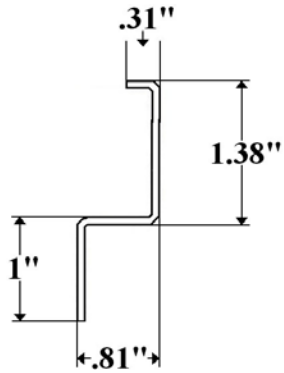
Part 03020R&L-Utilimaster Vertical Connector Aluminum Body 108"
