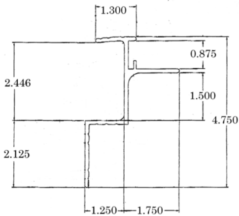
Part 3007- Utilimaster Top Rail New Style
