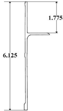
Part 3004- Utilimaster Bottom Rail From 2/98
