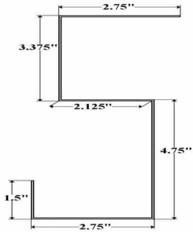
Part UT1- Utilimaster Rear Header
