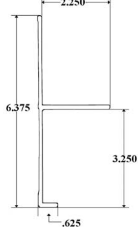
Part 3003- Utilimaster Bottom Rail Thru 1/98
