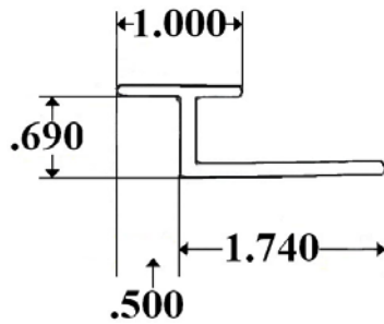
Part 03020R&L-Utilimaster Vertical Connector Aluminum Body 108"
