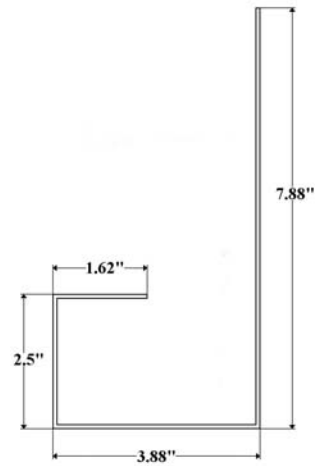
Part UT3 (108")- Utilimaster Rear Corner Post
